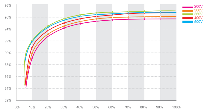
5k efficiency
